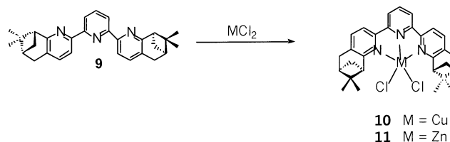
Scheme 2. Synthesis of the complexes
