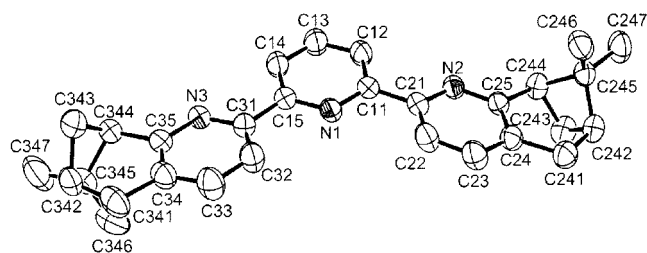
Figure 1. Molecular view of 9 with atom labelling scheme; ellipsoids represent 30% probability
