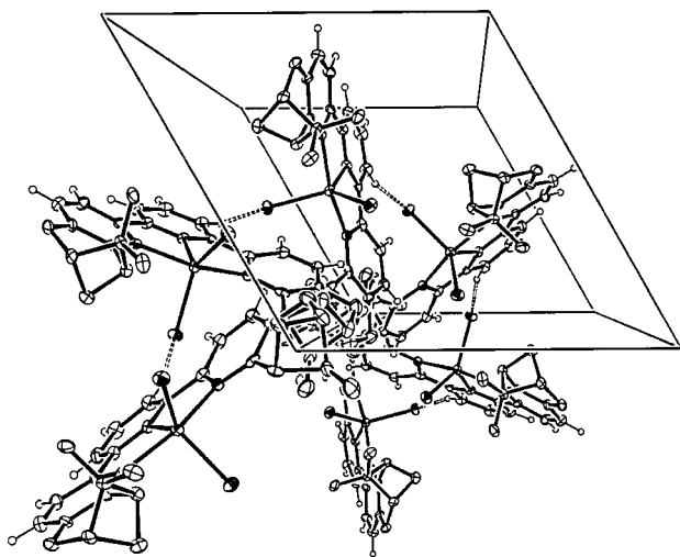
Figure 3. View along the 0 0 1 axis showing the right handed helix packing of the complexes around the 6 1 axes
