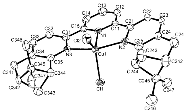
Figure 2. Molecular view of complex 10 with atom labelling scheme; ellipsoids are drawn at 30% probability
