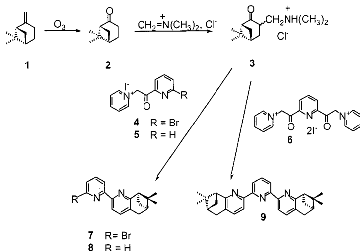
Scheme 1. Synthesis of the polypyridyl ligands
